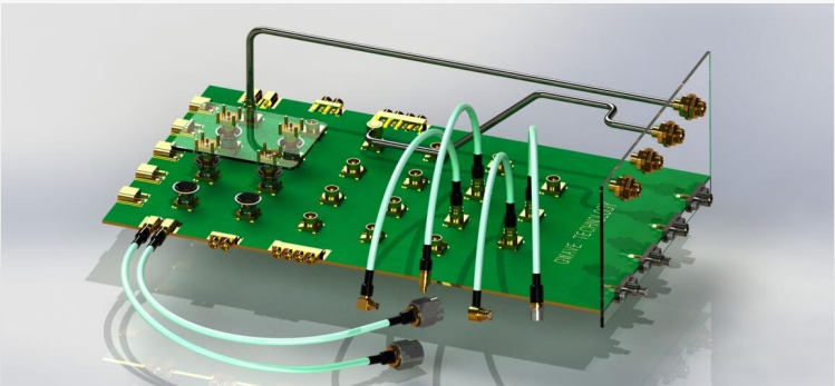
Board to board solution
